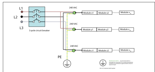
240V~ connection between phases (240V~ power grid)
