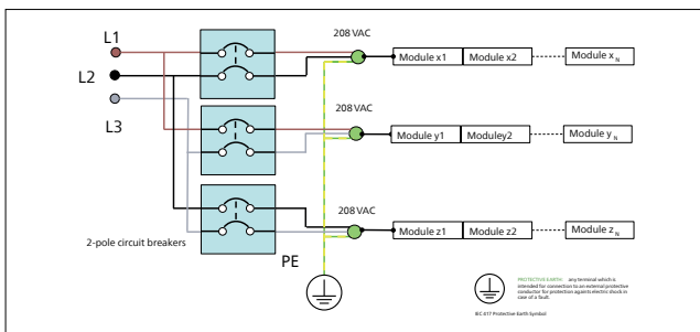
208V~ connection between phases (208V~ power grid)
