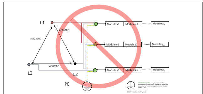
480V~ connection between phases (480V~ power grid)
