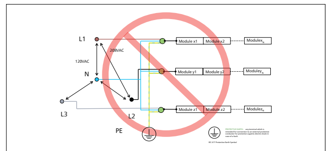
120V~ connection between neutral and phase (208V~ power grid)
