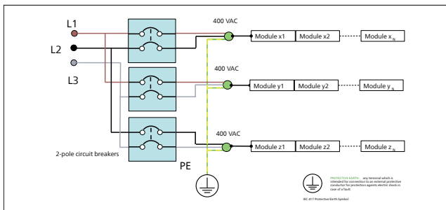
400 V~ connection between phases (400 V~ power grid).
